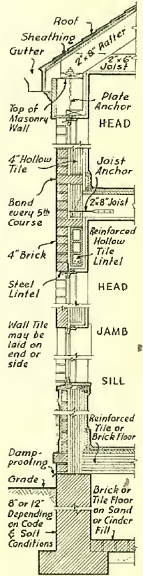
Wall Section
